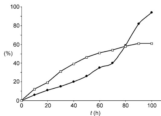
Figure 2. Evolution of the regioisomeric proportion 2a/3a relative to 2a under the usual conditions (Table 1, entry 6). ●: conversion, □: regioisomeric proportion.
