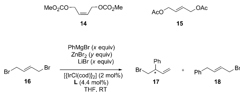
Scheme 7. Allylic arylation on a difunctionalized allylic substrate.
