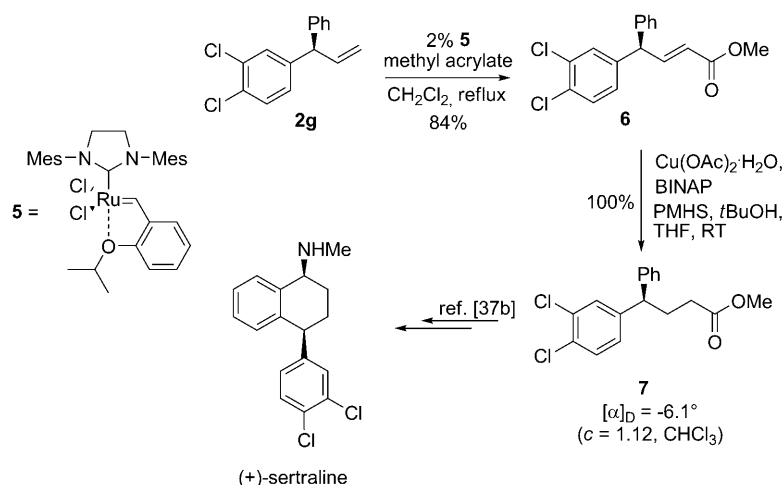
Scheme 4. Towards the enantioselective formal synthesis of (+)-sertraline.
