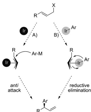
Figure 1. Two possible pathways explaining the product stereochemistry; A) anti attack pathway and B) reductive elimination pathway.
