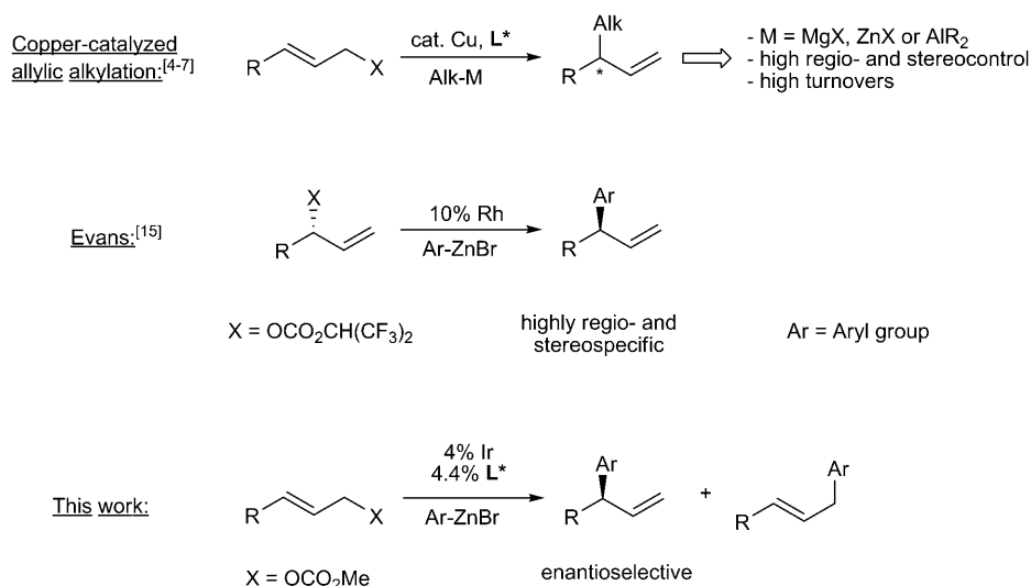
Scheme 1. Examples of allylic substitution reactions using nonstabilized nucleophiles.
