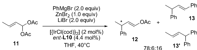
Scheme 6. Allylic arylation on a gem -difunctionalized substrate.
