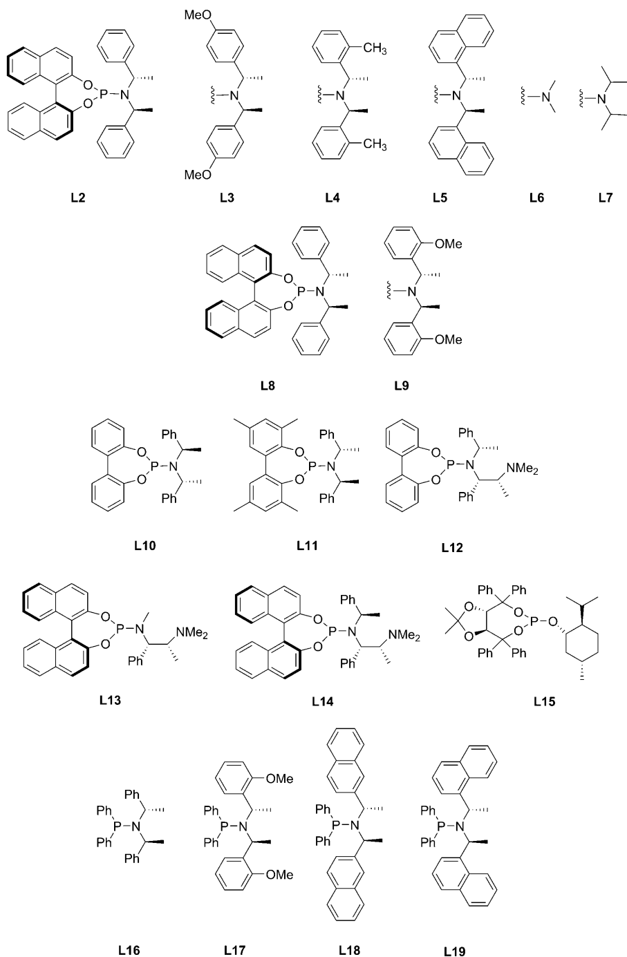
Scheme 3. Chiral ligands used in this study.
