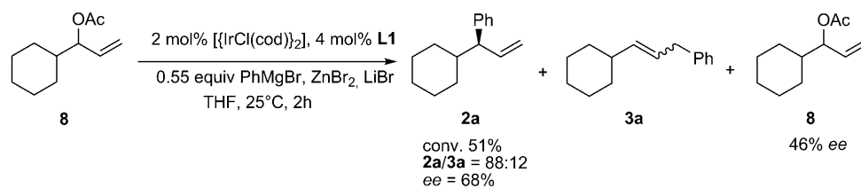
Scheme 5. Allylic arylation under kinetic resolution conditions.
