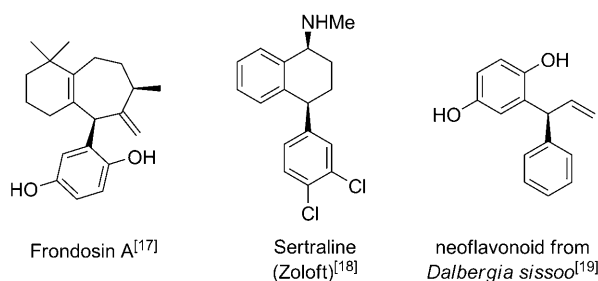
Scheme 2. Natural and non-natural biologically active compounds that could arise from the asymmetric allylic transfer of an aryl group.
